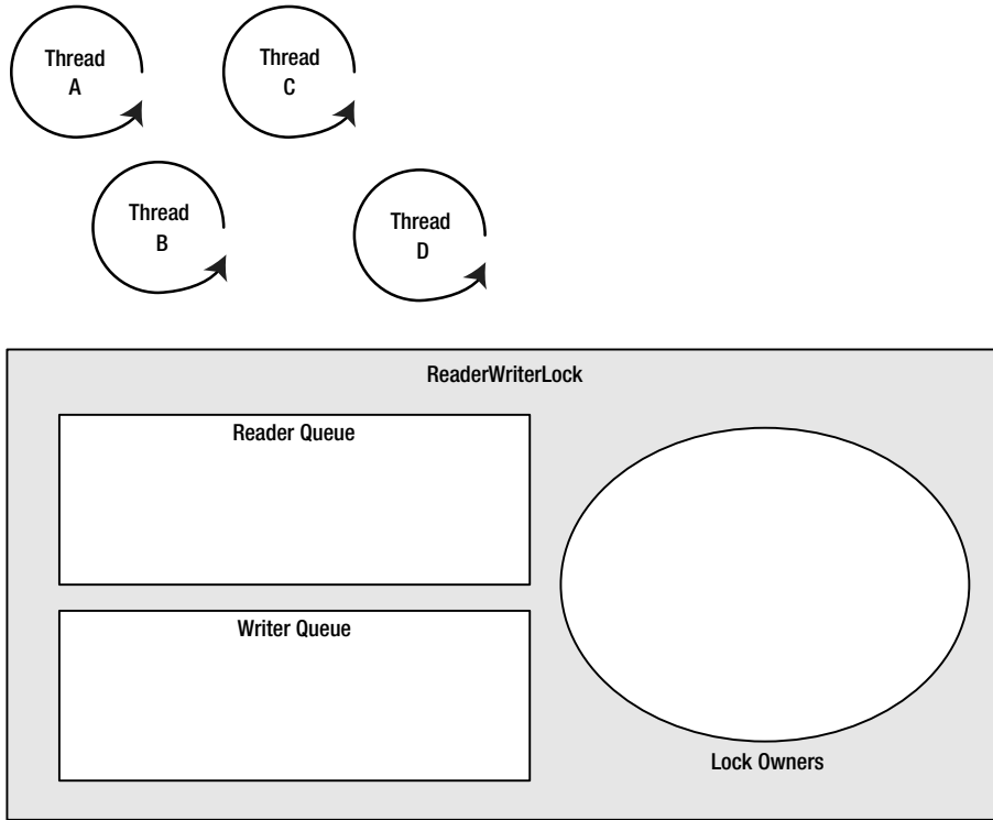
Figure 12-2. Unutilized ReaderWriterLock
