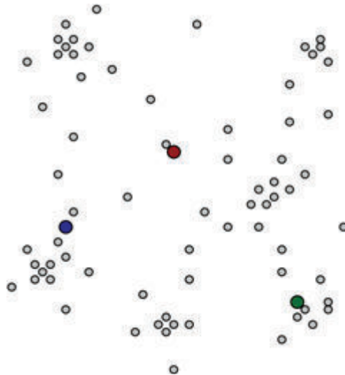
FIGURE 4-2 Initial starting points for the centroids
