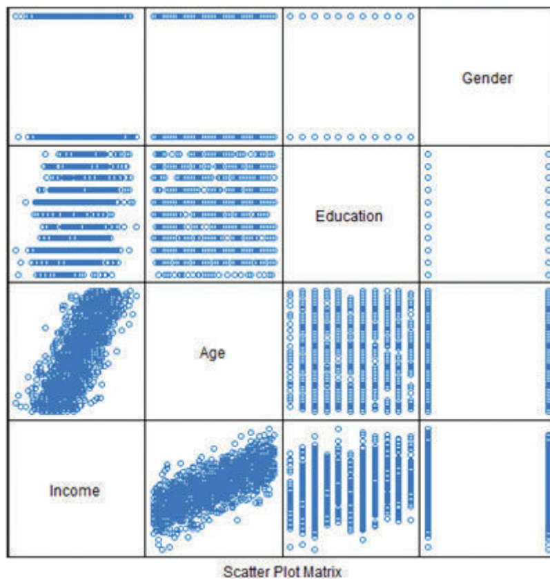
FIGURE 6-4 Scatterplot matrix of the variables
