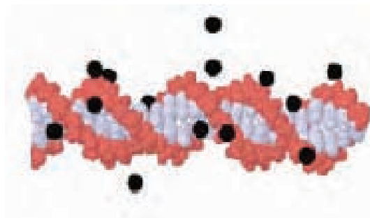
Figure 2.6. Counterions surrounding DNA in solution. The counterions can form periodic structures along their associated DNA molecules. (Reprinted with permission from [6], copyright 2003 by the American Physical Society.)
